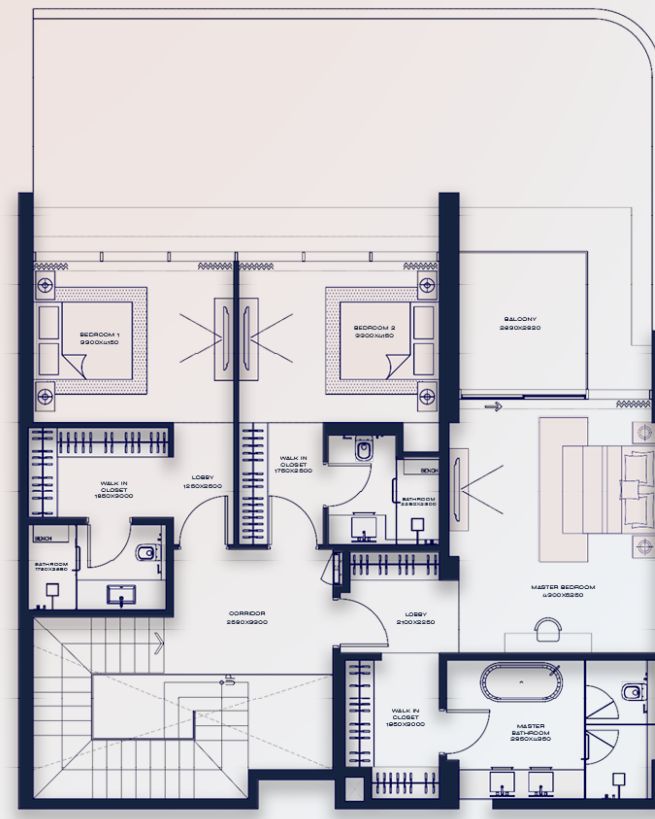
LAYOUT 2
