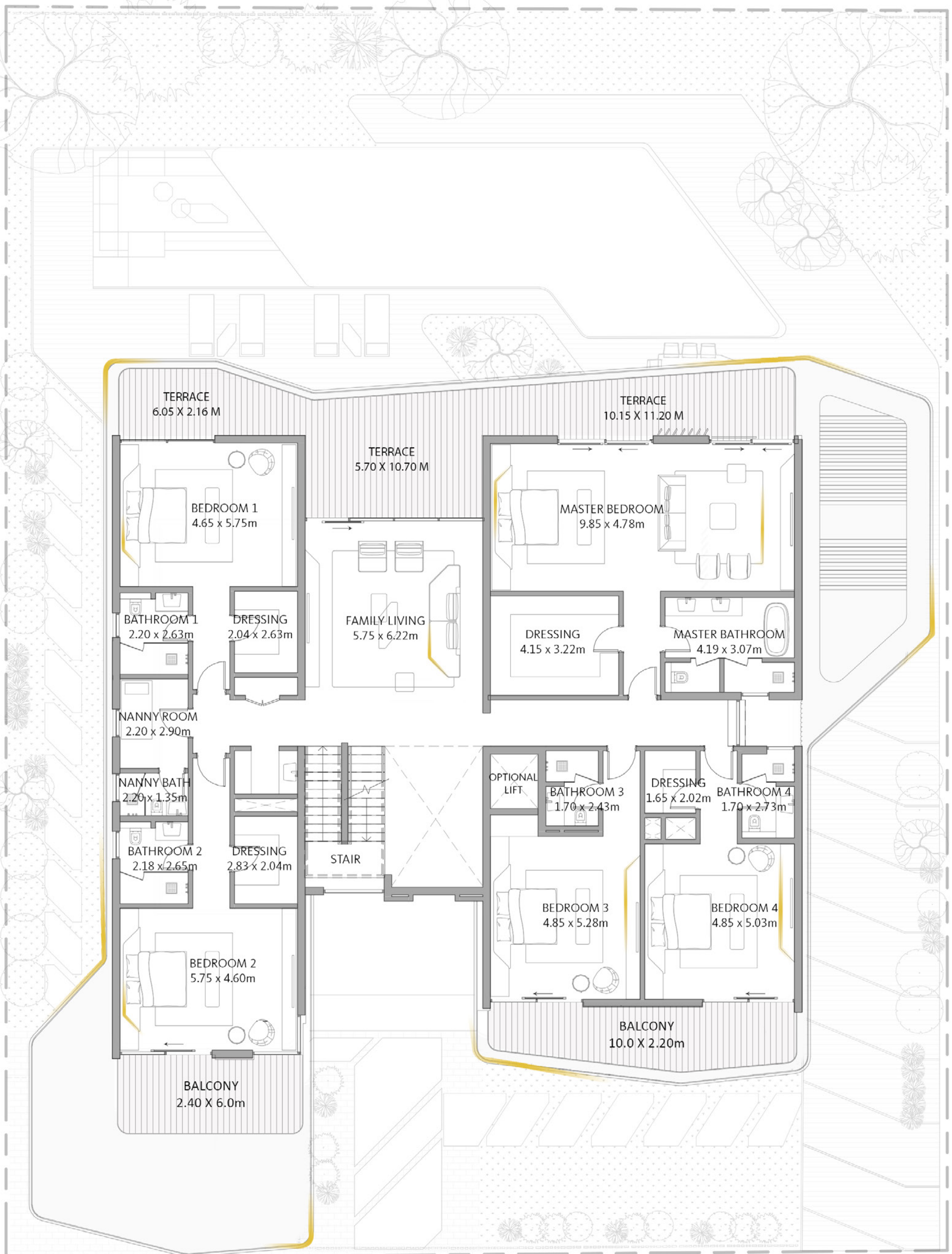
FIRST FLOOR
