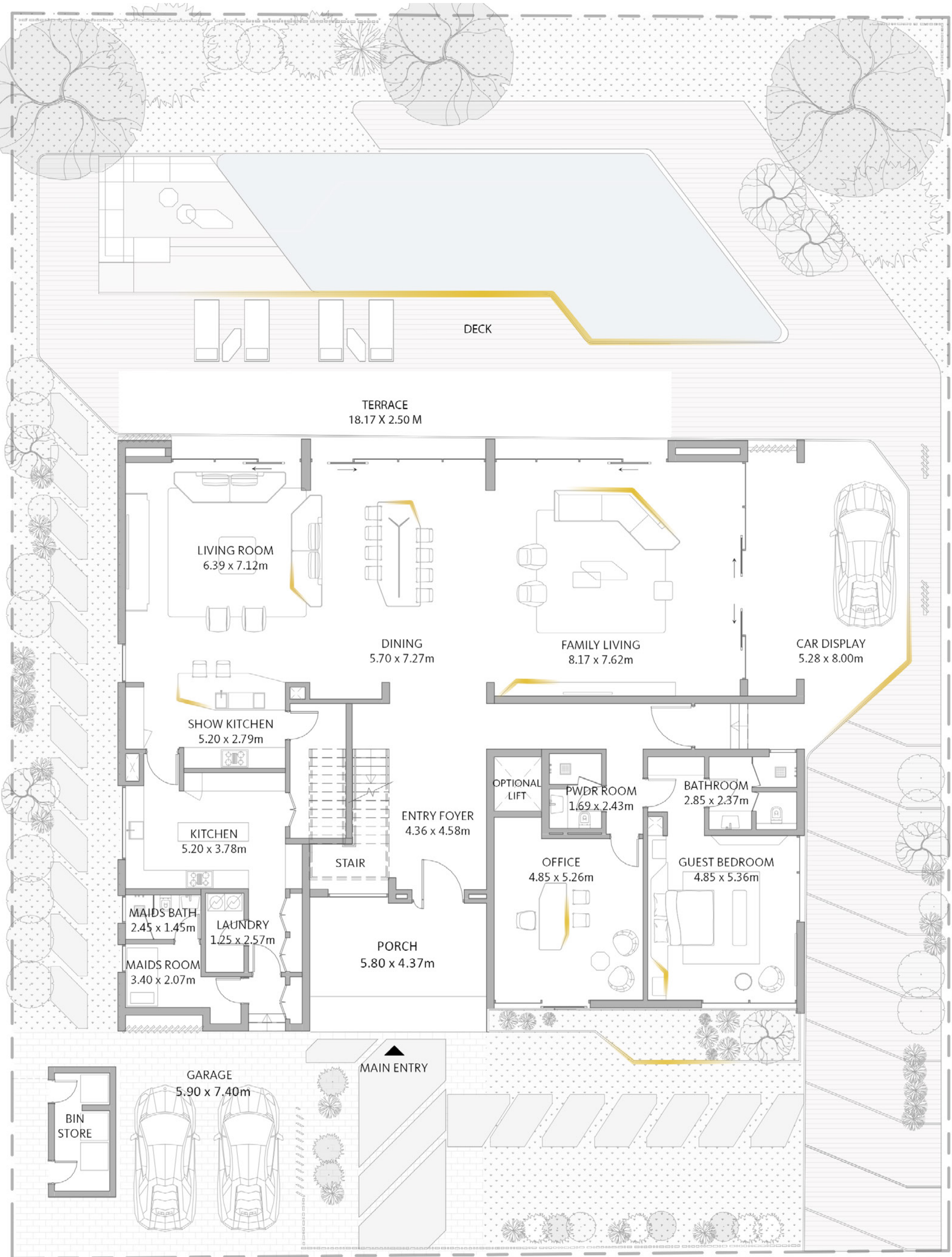
GROUND FLOOR
