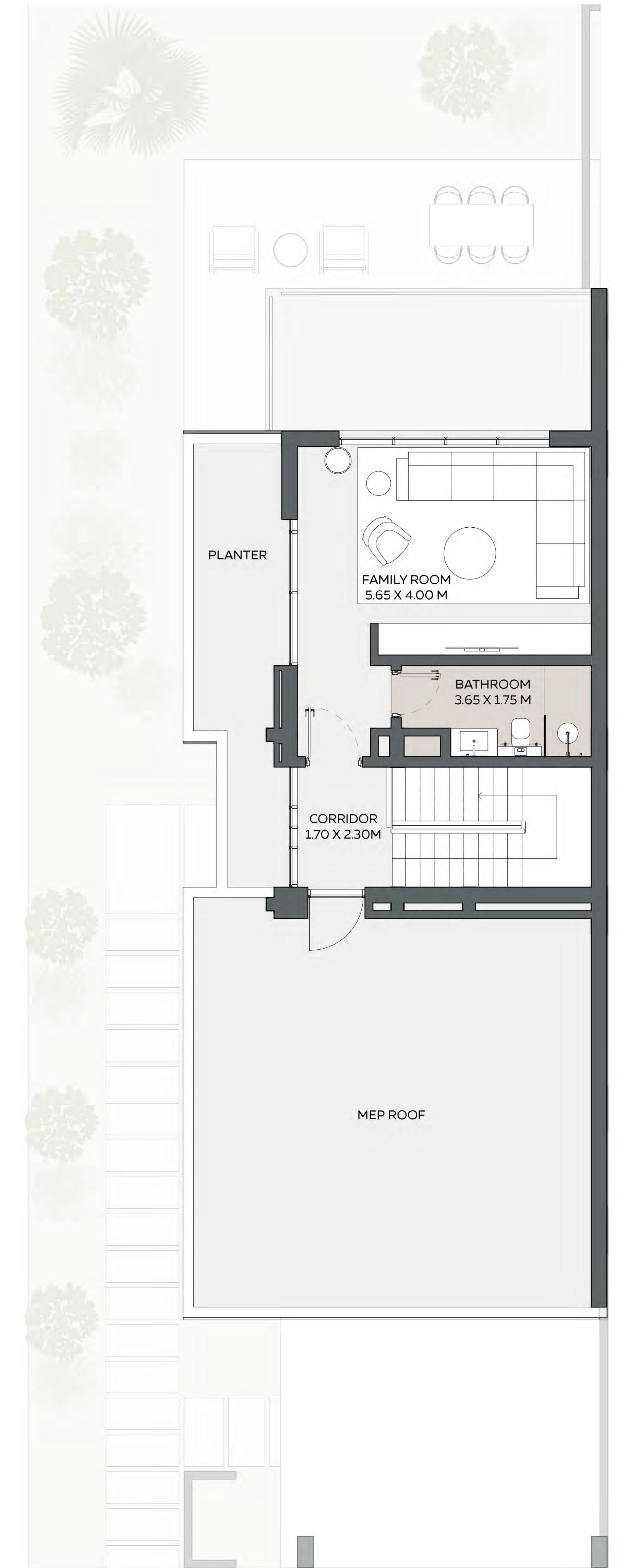
ROOF FLOOR
