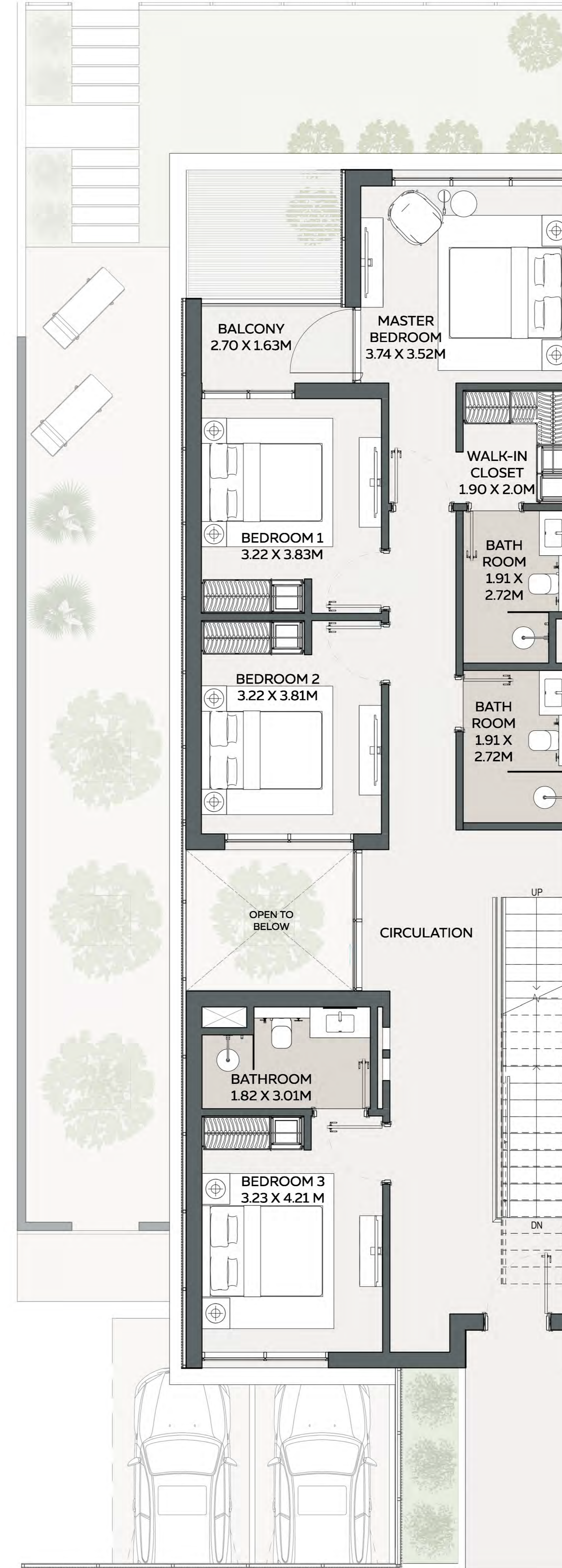
GROUND FLOOR
