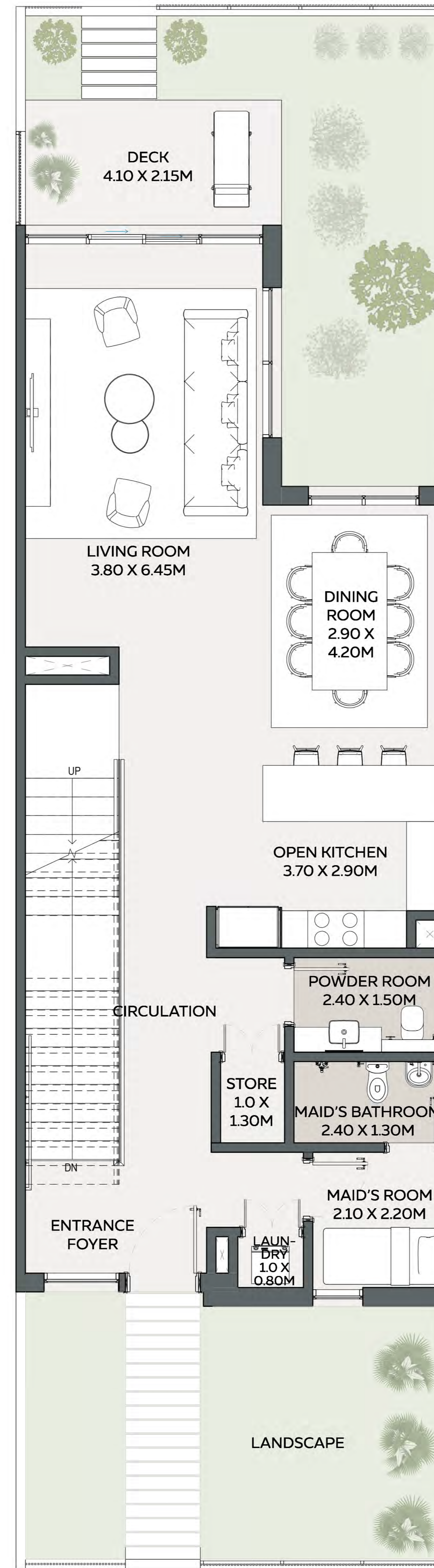
GROUND FLOOR
