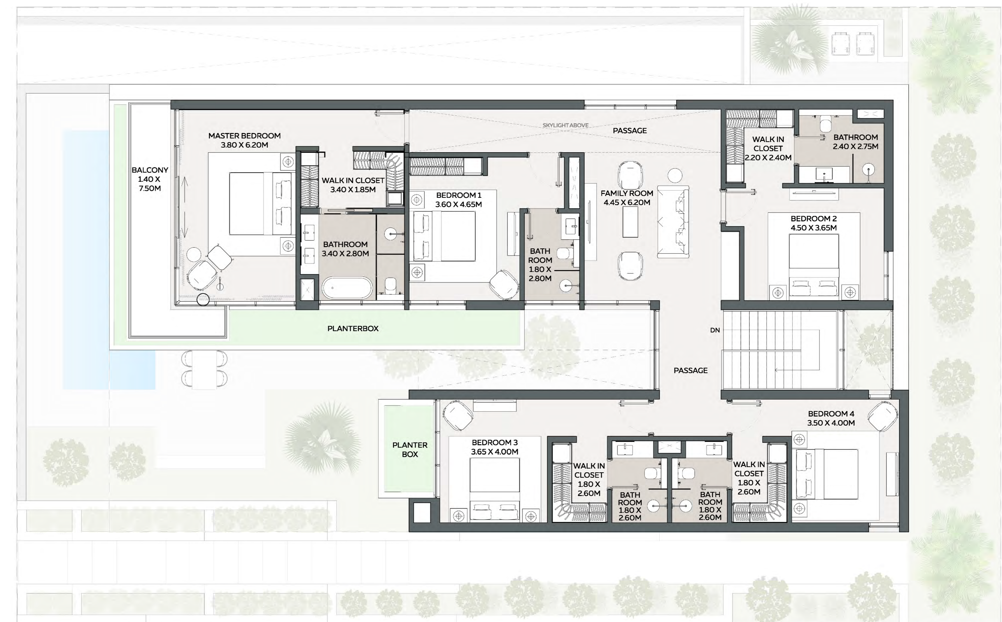
FIRST FLOOR
