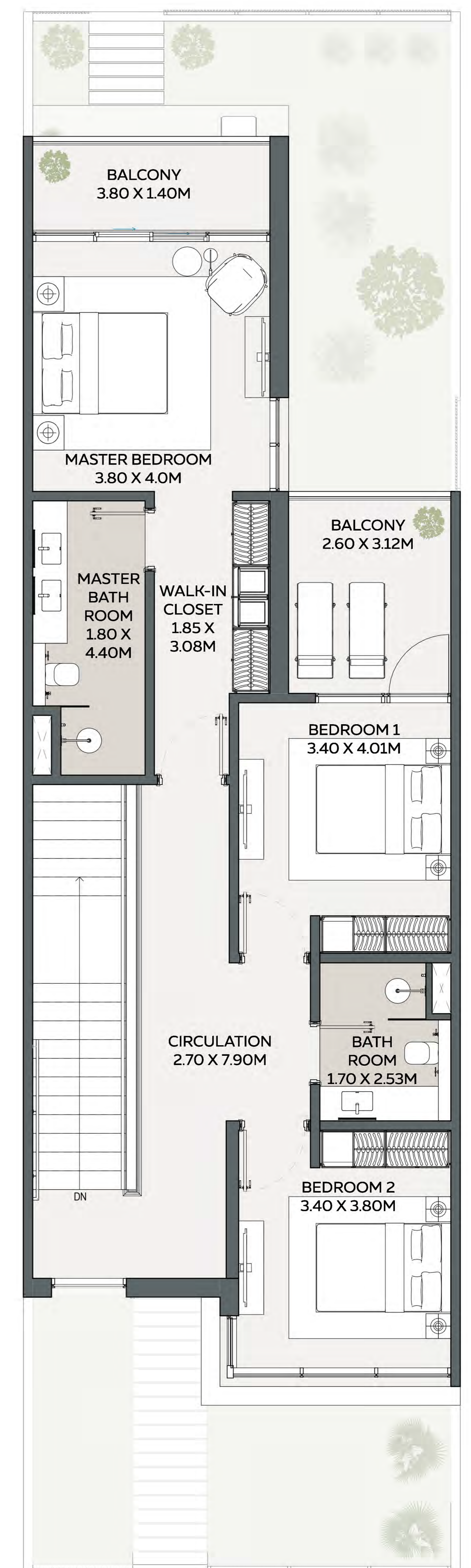
FIRST FLOOR
