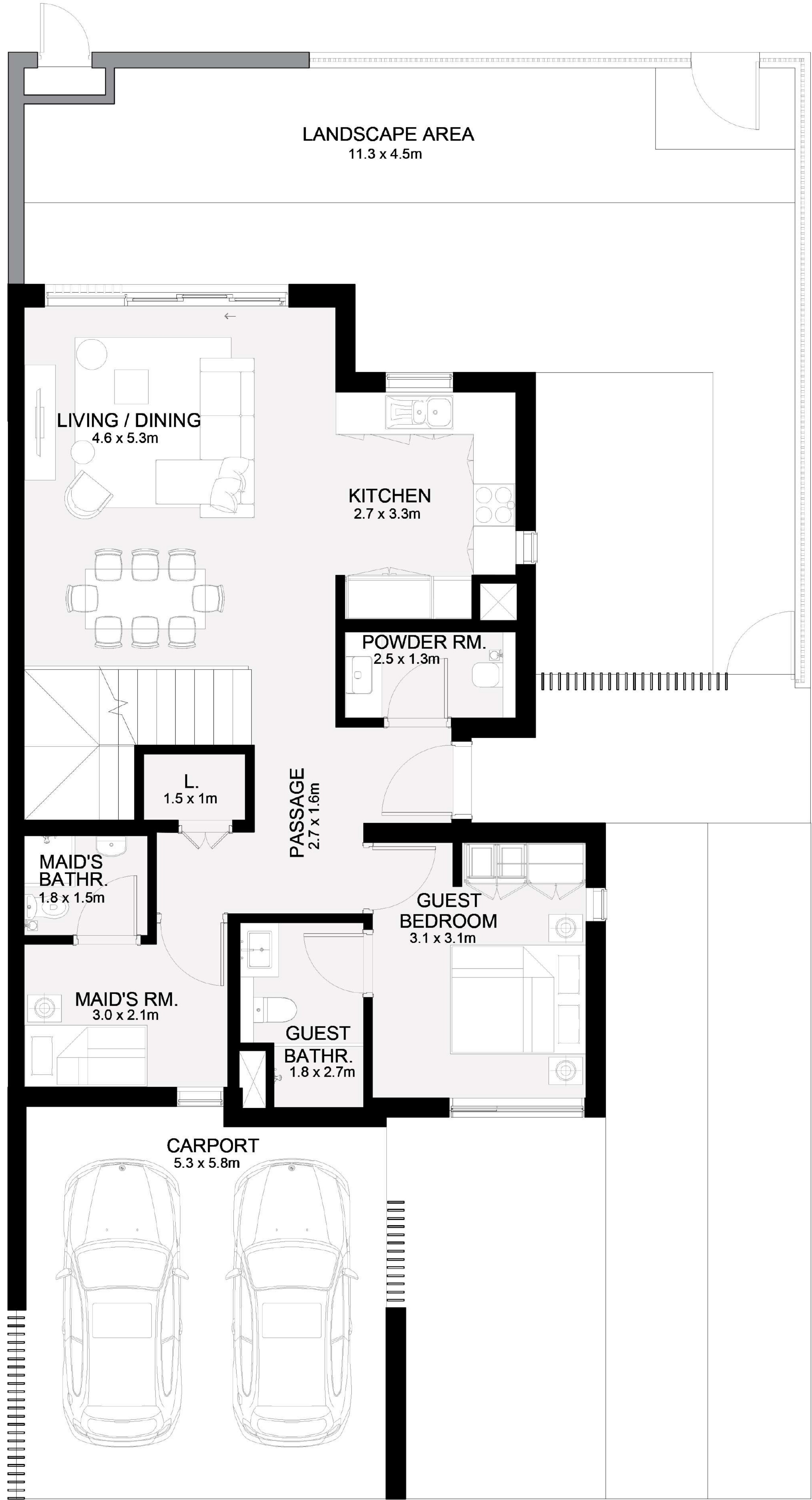
GROUND FLOOR
